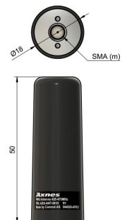
Outline Dimensions (mm)
