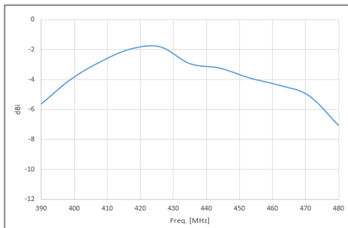
Gain dBi (horizon)
