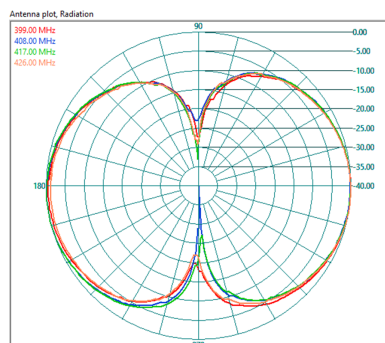
Radiation Pattern (typical)
