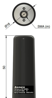
Outline Dimensions (mm)
