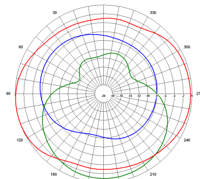
Typical azimuth radiation pattern with two separate antennas
