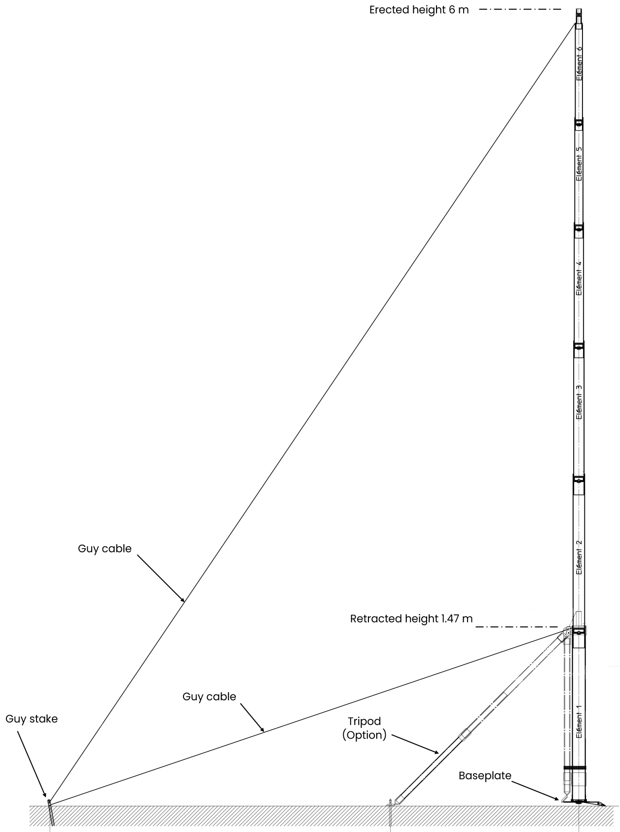
Standard installation : ground mounted with guy cables
