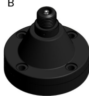
B NATO 4-hole Rigid (no spring) 4 x M10 or 3/8" Bolts on 114 mm PCD Base diameter 140 mm
