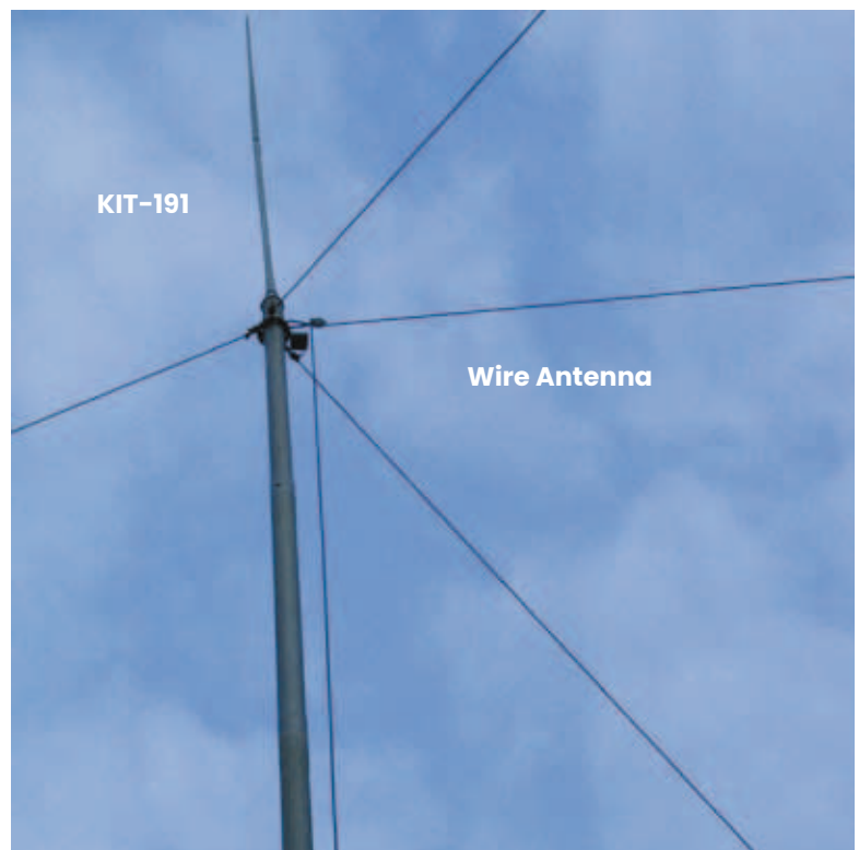
Example of a Two Antenna Installation
